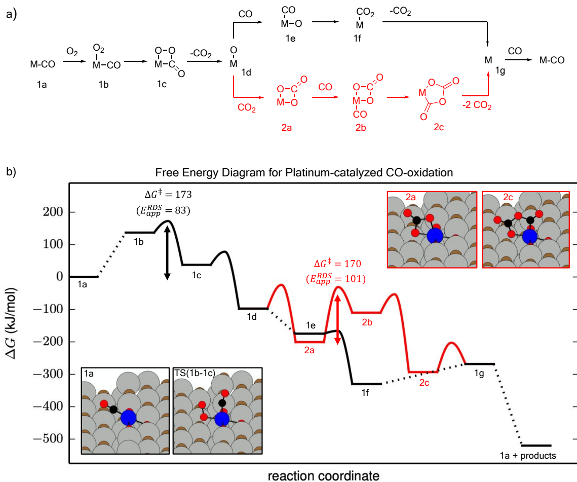
Figure 5: Mechanism investigated with DFT-calculations for Pt. a) Scheme for CO-oxidation mechanism starting from the metal carbonyl. b) Free energy diagram computed for Pt at 573 K and 1 bar reference pressure for the mechanisms shown in a) using the same labels. The two highest barriers are indicated and the values given in kJ/mol. Additionally, apparent activation energies as derived from these barriers and the rate-determining step (RDS) approximation are provided (see section 2 in the Supporting Information for the corresponding Arrhenius plots). Insets depict the atomic structures of important intermediates and transition states (color code: Mg: gray, lattice-O: brown, O: red, C: black, Pt: blue).
